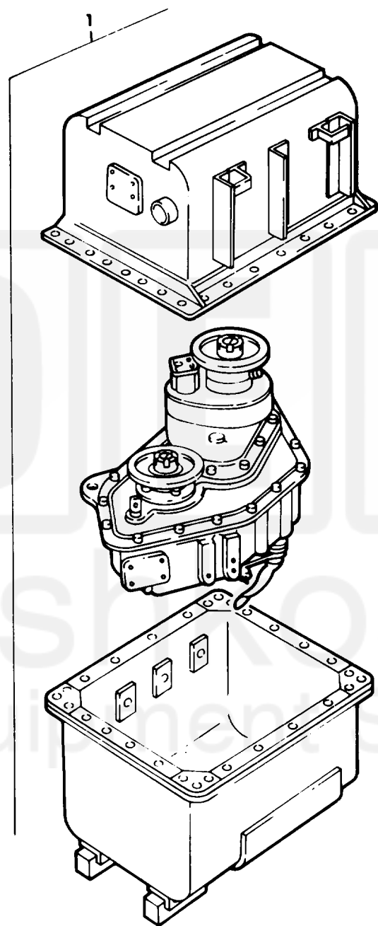
Figure 141. Transfer and Container Assembly.
